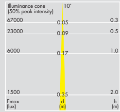
Lamp: Decostar IRC 50W 10°
