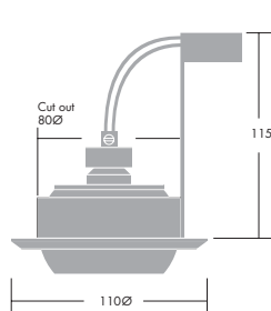
Eyeball +/- 40°
