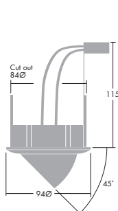
Out-swivelling 0-45°
