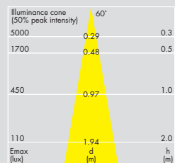
Lamp: Decostar IRC 50W 60°
