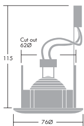
Fixed version
