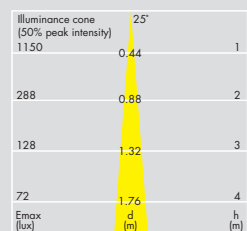
Lamp: 50W PAR16 25°
