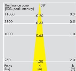
Lamp: Decostar IRC 50W 38°
