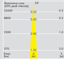
Lamp: Decostar IRC 50W 24°
